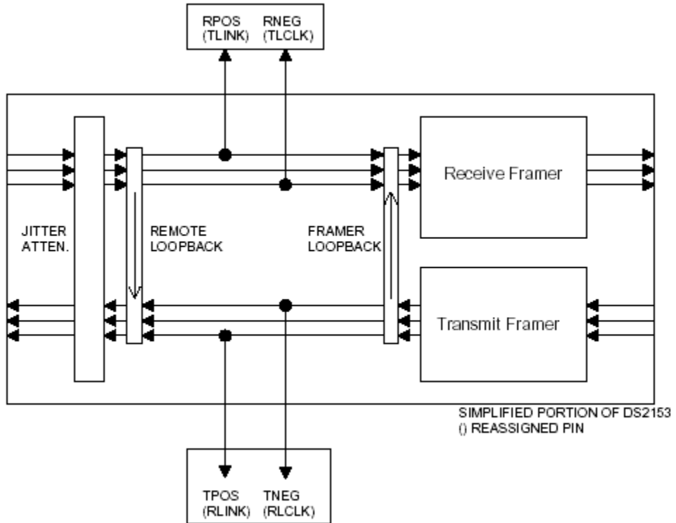
Mode 3: DS2153 Special Mode to Tap the Transmit & Receive Bipolar Data
