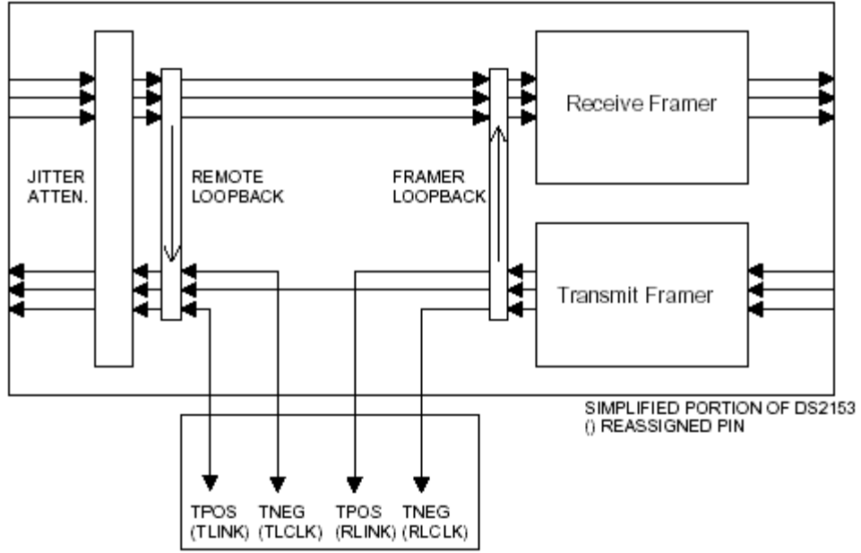
Mode 2: DS2153 Special Mode to Allow Access to Transmit Bipolar Data
